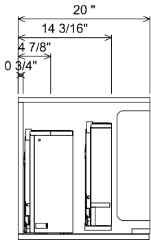
AT CENTER SINK SECTION
